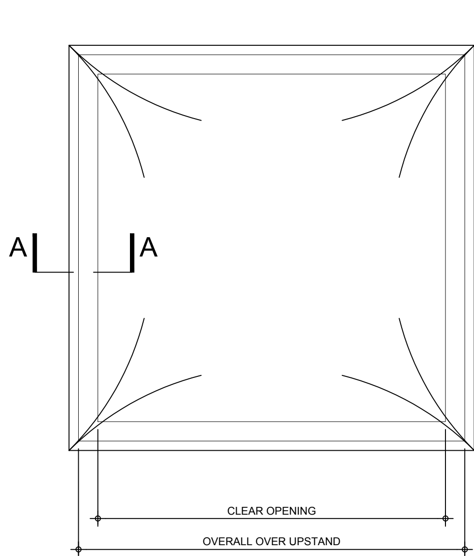
PLAN ON SINGLE SKIN DOME ROOFLIGHT (1No. REQUIRED AS SHOWN)
