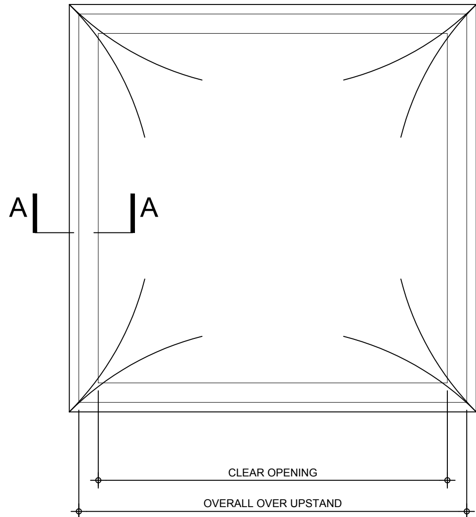
PLAN ON TRIPLE SKIN DOME ROOFLIGHT (1No. REQUIRED AS SHOWN)
